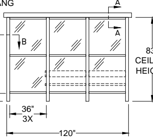
ELEVATION C
