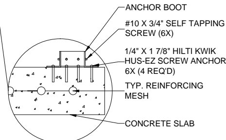
ANCHORING DETAIL
